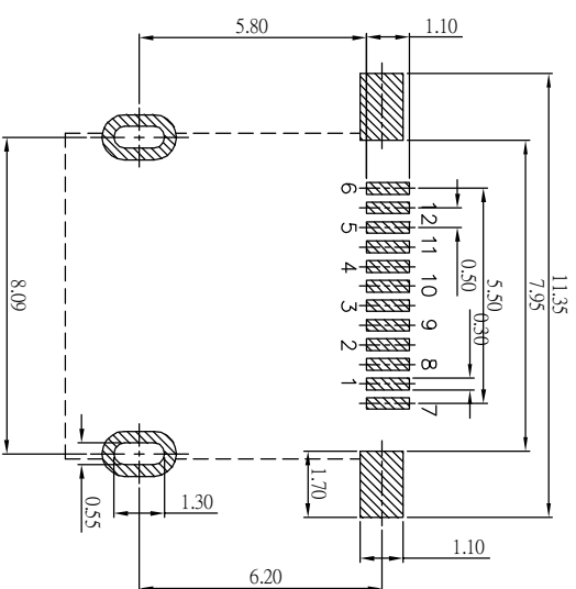
RECOMMENDED P.C.B. LAYOUT TOLERANCE: ±0.05 TOP VIEW
