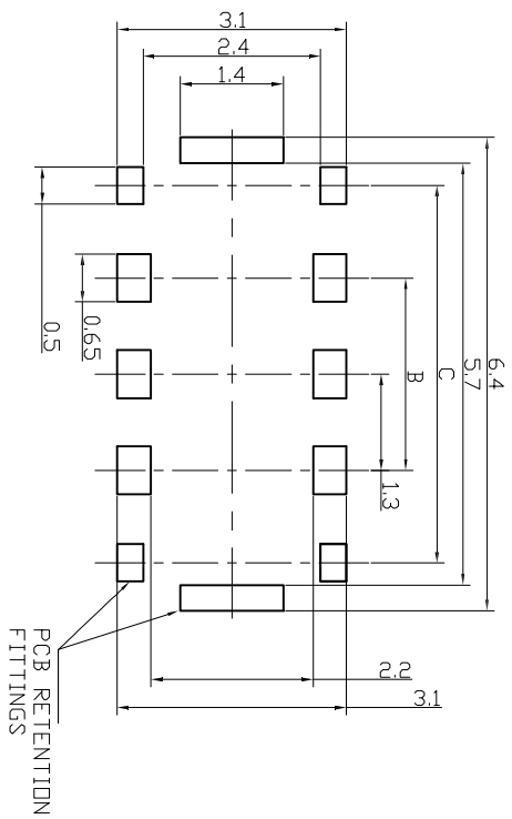
PCB LAYOUT
